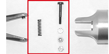
BA-HR5 - Blade Mounting
